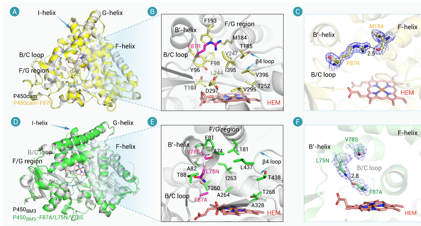
Figure 3. Structural analysis of the substrate-binding pockets in P450 variants (A) Superimposition of the substrate-free structures of P450cam-F87R (yellow, PDB ID: 25BV) with P450cam-WT (gray, PDB ID: 2A1M) 34 . (B) Detailed view of the active pocket of P450cam-F87R, with the surrounding secondary structural elements labeled. (C) Conformational analysis of the mutated residue in P450cam-F87R. (D) Structural overlay of P450 BM3 -F87A/L75N/V78S (green, PDB ID: 9L7U) with the wild-type P450 BM3 (gray, PDB ID: 1Z09) 35 . (E) Detailed view of the active pocket of P450 BM3 -F87A/L75N/V78S, with the surrounding secondary structural elements labeled. (F) Conformational analysis of mutated residues in P450 BM3 -F87A/L75N/V78S.
