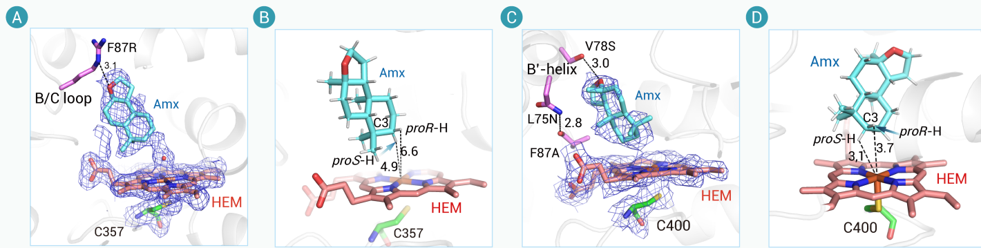
Figure 4. Structural basis for the regio- and stereoselectivity of P450 variants toward (–)-ambroxide (A) Electron density map of (–)-ambroxide in the substrate binding pocket of P450cam-F87R (PDB ID: 9L7R). (B) The distances between the two C–H bonds at the C3 position of the substrate and the heme-iron in the 9L7R structure. (C) Electron density map of (–)-ambroxide in the substrate binding pocket of P450 BM3 -F87A/L75N/V78S. (D) The distances between the two C–H bonds at the C3 position of the substrate and the heme-iron in the 9L7U structure. The 2mF_o - DF_c densities for the ligand, heme, and residues are outlined in blue at a 1.0 \sigma level. The distances are indicated in angstroms.
