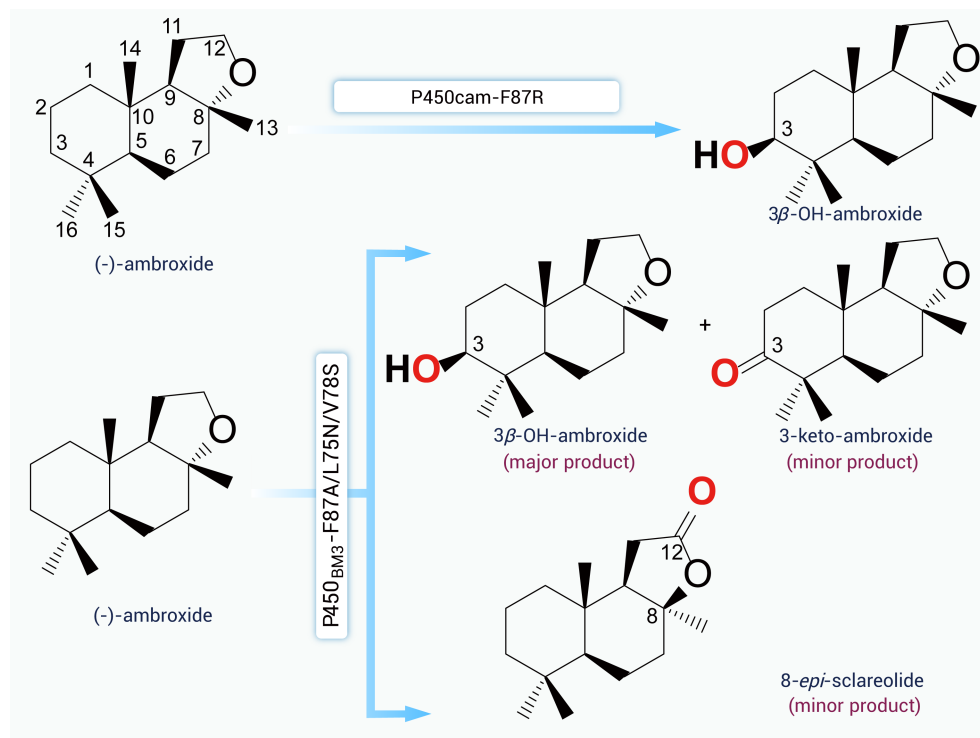
Figure 1. Schematic oxidative reactions of (-)-ambroxide The reaction pathways illustrate that P450cam and P450 BM3 variants exhibit convergent 3β-hydroxylation activity.
